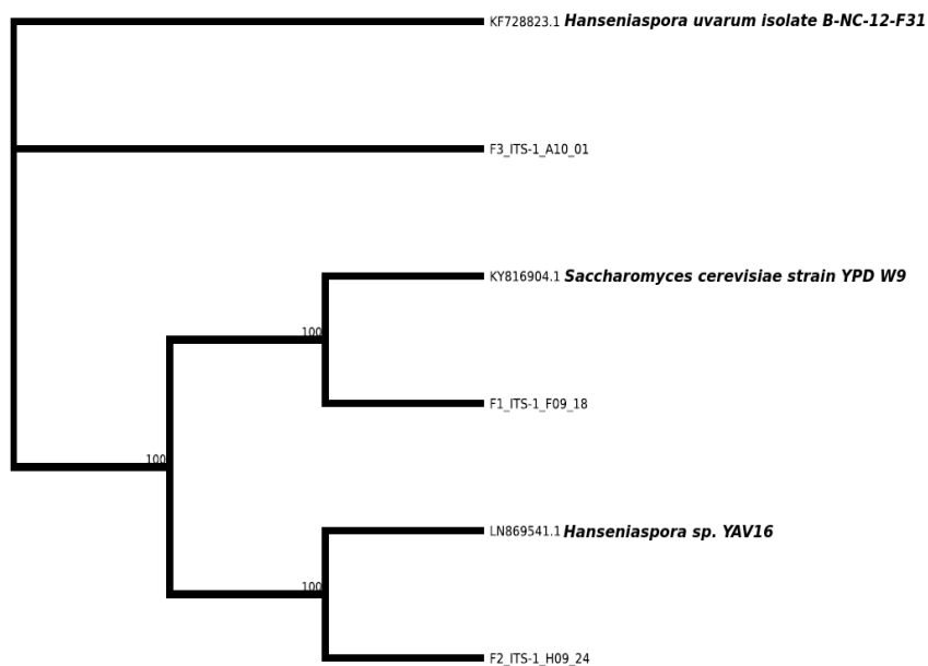
Fig. 2. Phylogenetic characteristics of evolutionary relationship between the fungal isolates F1: Saccharomyces cerevisiae YPD W9; F2: Hanseniaspora sp. YAV 16 F3: Hanseniaspora uvarum B-NC-12-F31
